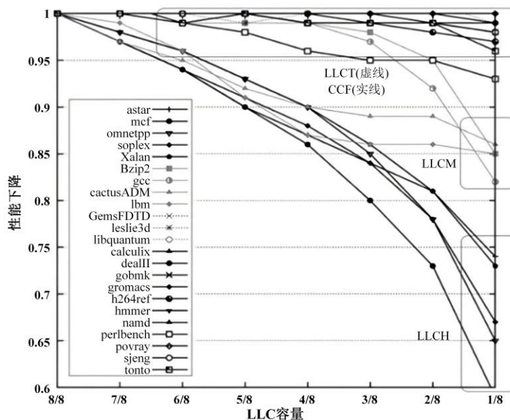
Fig.10 The relationship between cache capacity and performance
