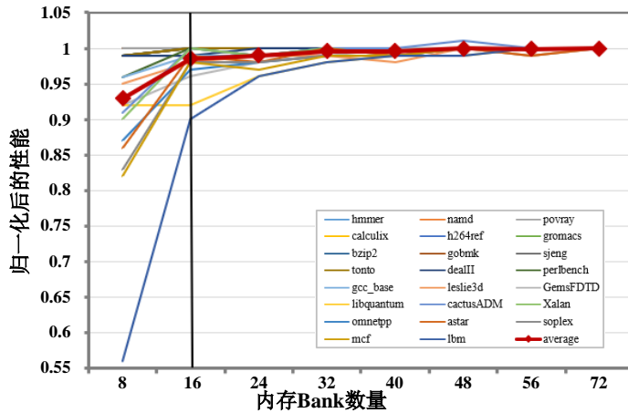
Fig. 3 Relationship between memory bank capacity and performance of a single program [5]
