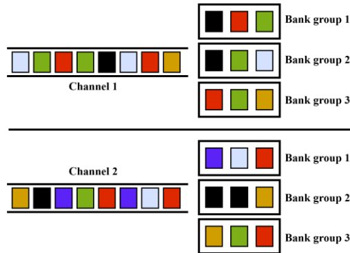
Fig. 5 Interleaving memory access across the memory channels among programs
