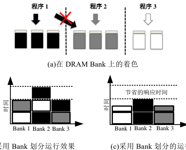
Fig.2 Page-coloring on DRAM bank (BPM) and performance w/ and w/o BPM
