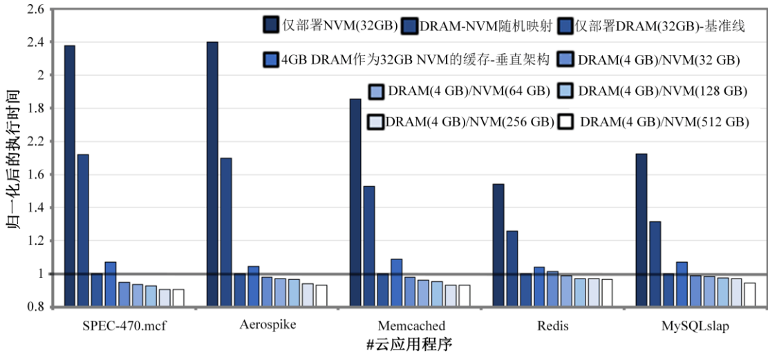
Fig. 15 Normalized execution time of cloud computing applications
