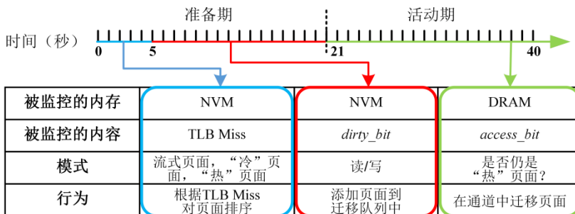
Fig. 14 HyMM’s general scheduling logic
